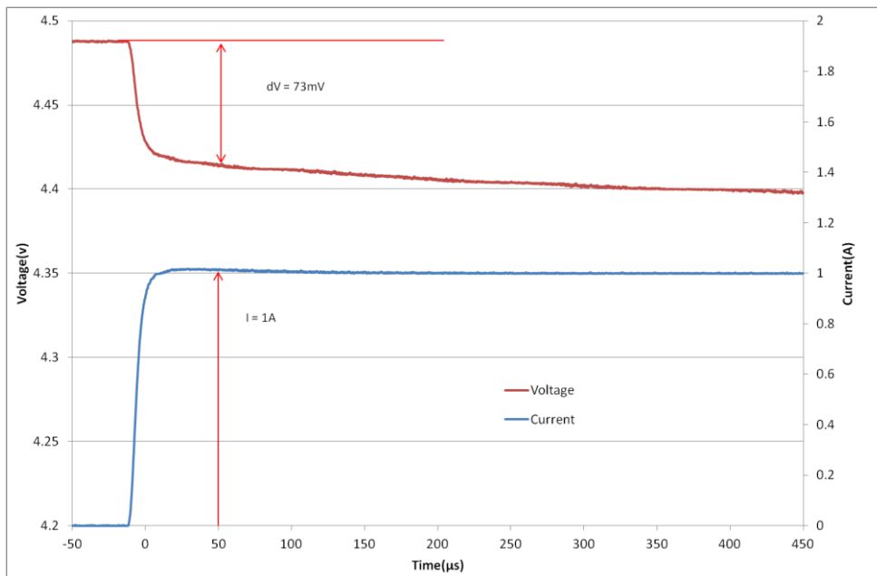
Fig 3: Measurement of ESR for a GA209
