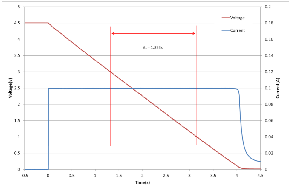
Fig 2: Measurement of DC Capacitance for a GA209
