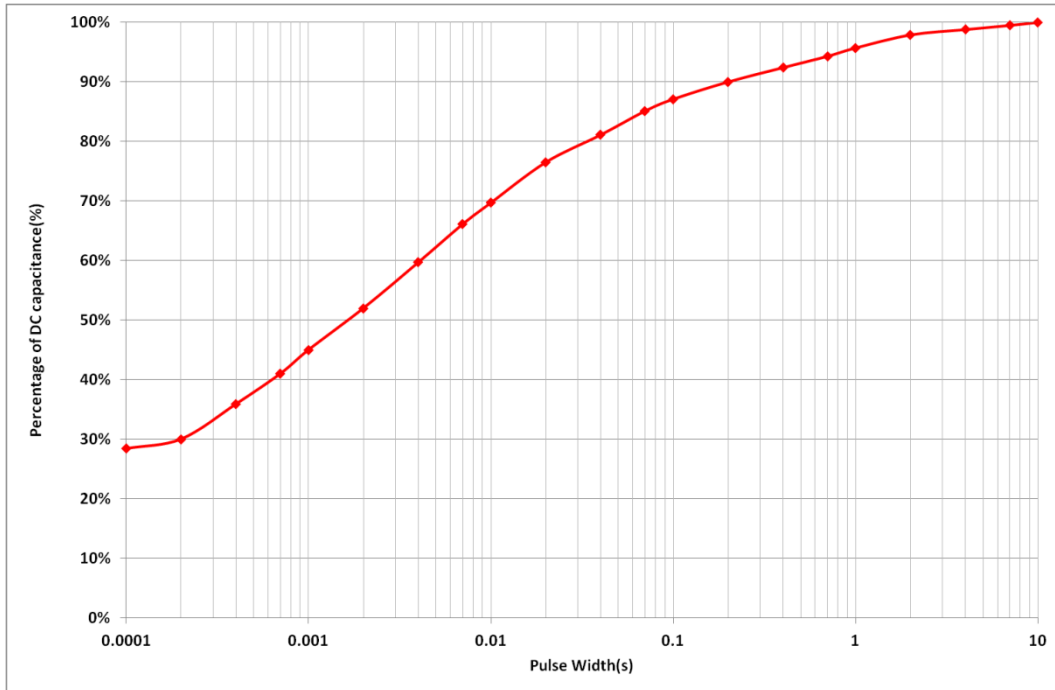
Fig 4: Effective Capacitance
