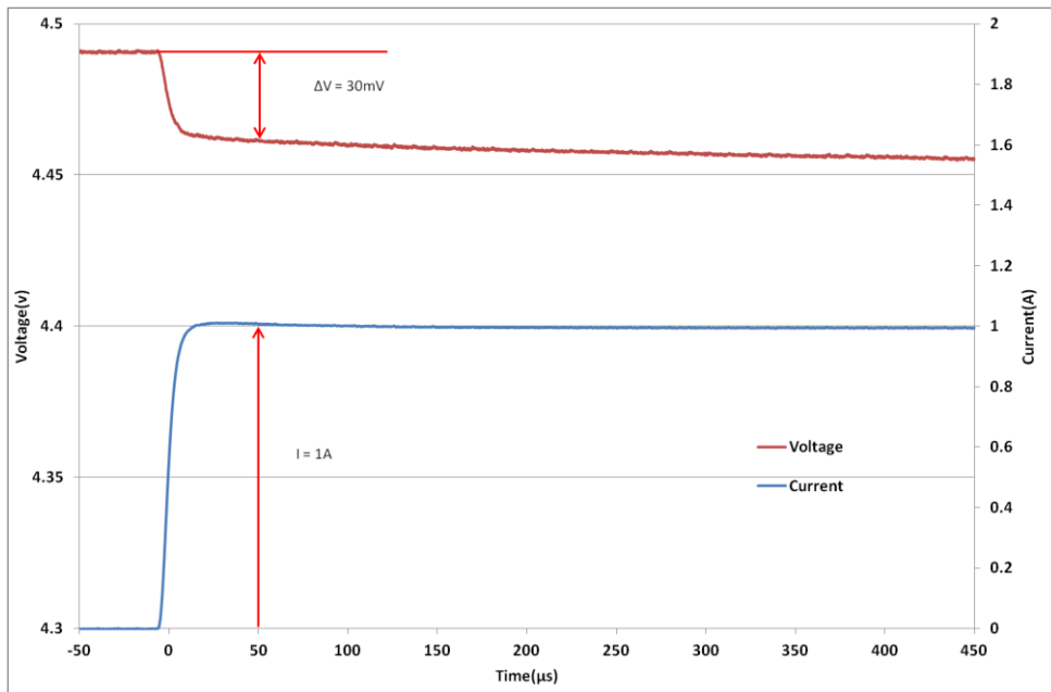
Fig 3: Measurement of ESR for a GS203
