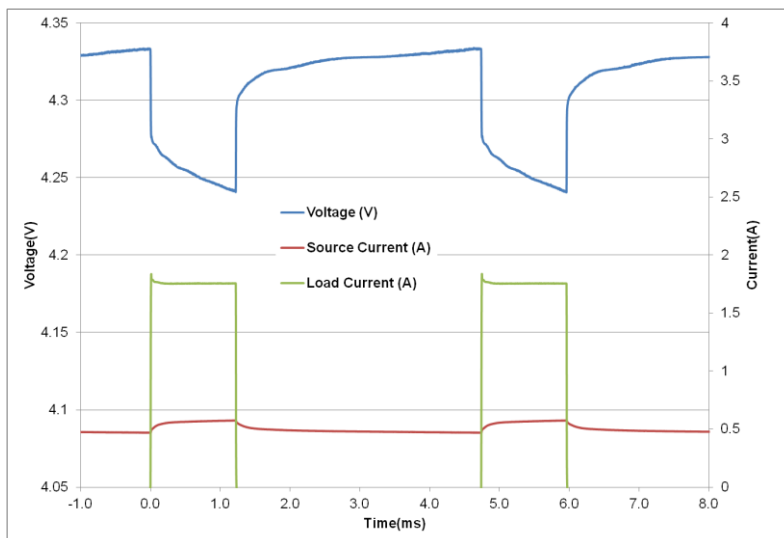
Fig 5: GW201 Pulse Response with GPRS Class 10 Pulse Train
