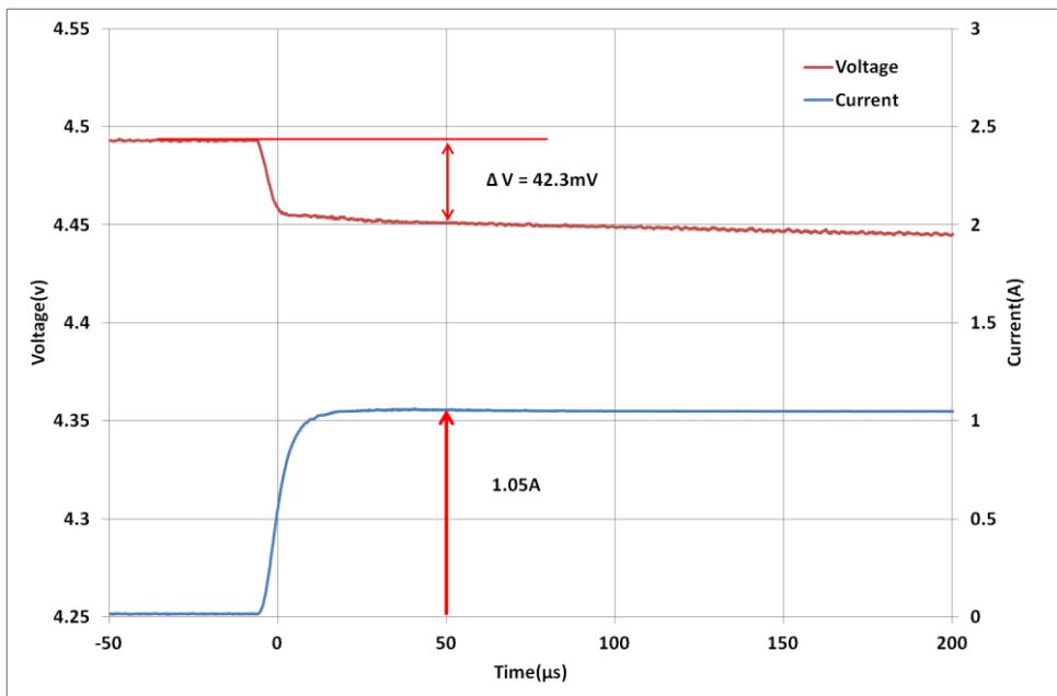
Fig 3: Measurement of ESR for a GW201
