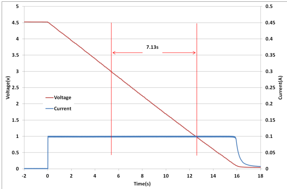
Fig 2: Measurement of DC Capacitance for a GW201
