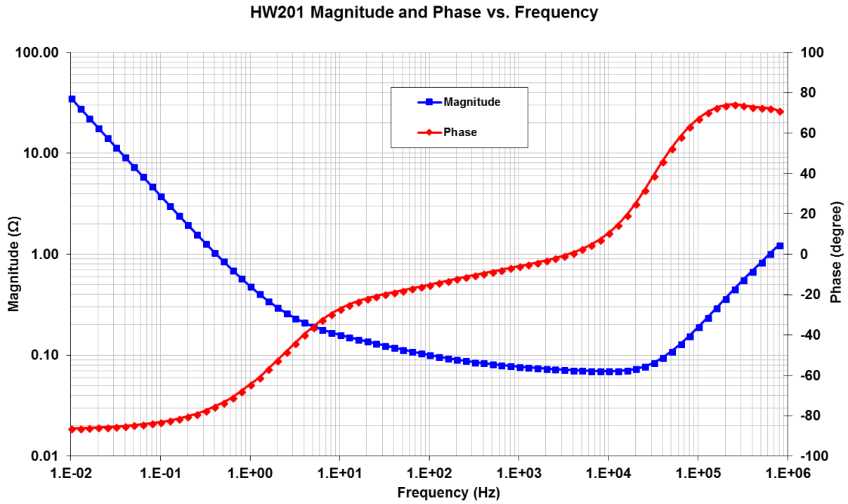
Fig 8: Frequency Response of Impedance (biased at 5.5V with a 50mV test signal)
