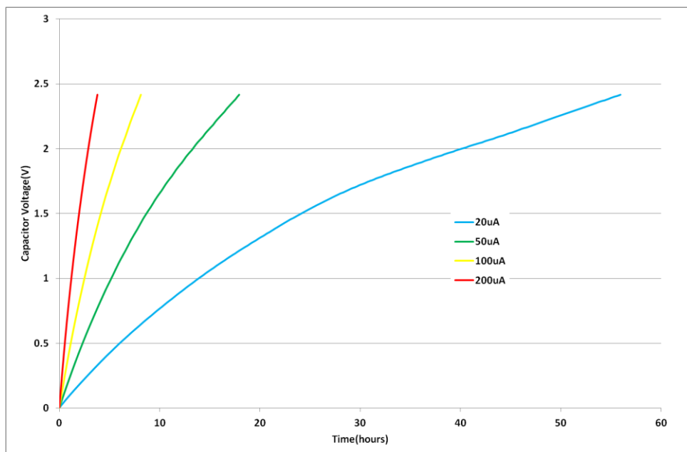
Fig 11: Charging an HW101 with low current
