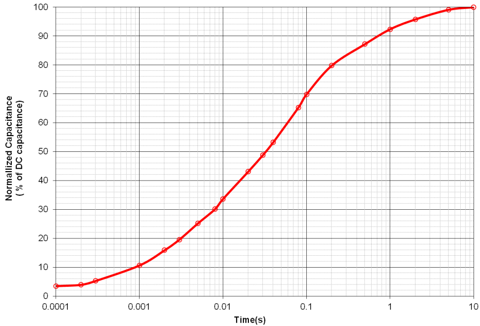
Figure 4: Effective Capacitance
