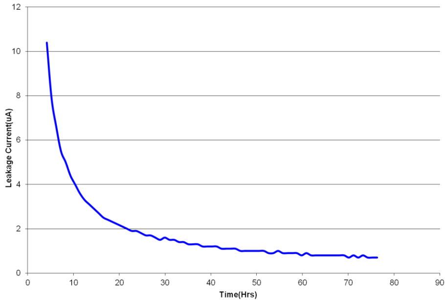
Fig 10: Leakage Current
